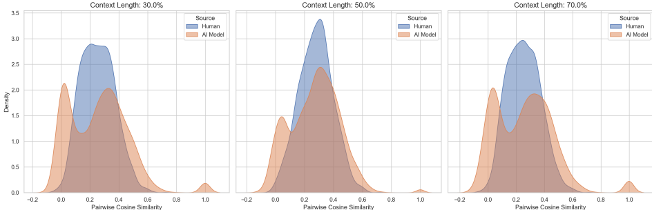
Figure 2: Distribution of cosine similarities between BGE text embeddings of human vs model ShortStories corpora. The LLM corpora vary in the percentage of the story they complete: 30%-70%.
